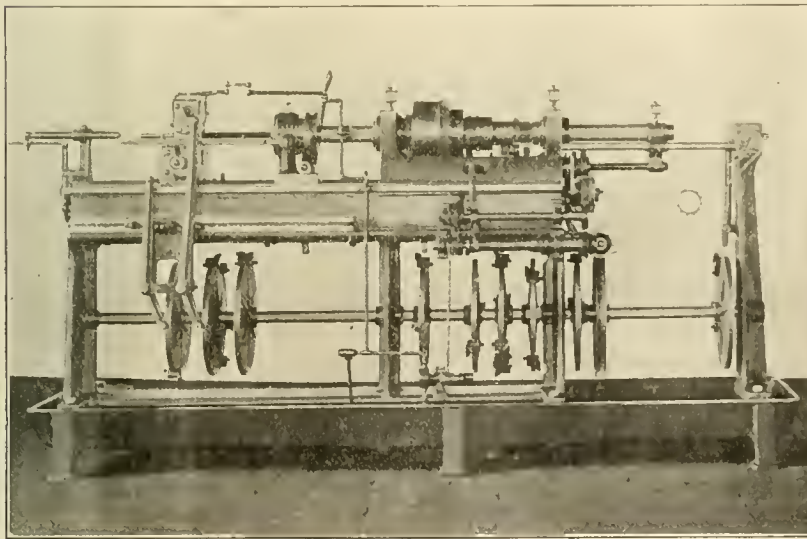
BACK OF EPRIGHT'S AUTOMATIC STAYBOLT CUTTER.
